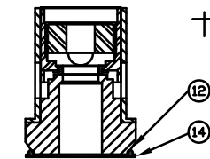
INNER VALVE UNIT (.500 & .625)
