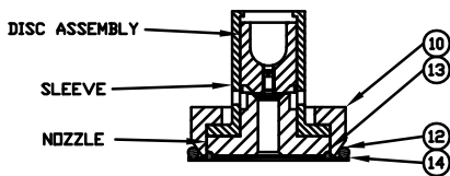
INNER VALVE UNIT WITH RETAINER RING (.125, .187, .250, & .375)
