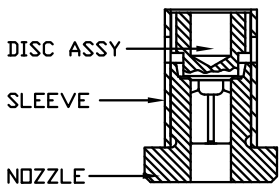
INNER VALVE UNIT DETAIL METAL SEAT
