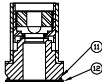
INNER VALVE UNIT (.500 & .625)
