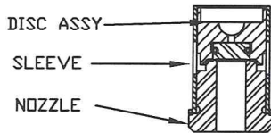
INNER VALVE UNIT DETAIL .500
