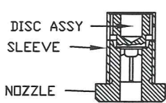
INNER VALVE UNIT DETAIL .375 & .437
